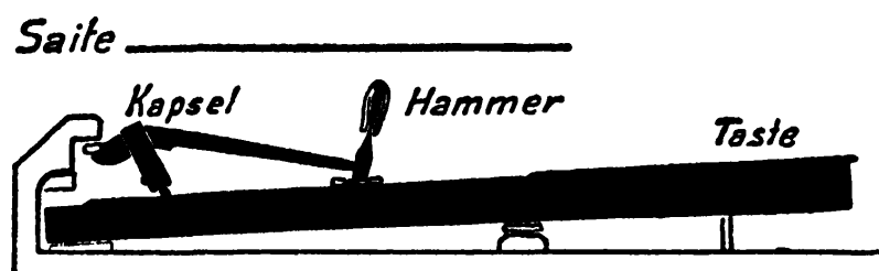
FIGURE 122. German Prellmechanik without escapement; del. Carmina Manger.
